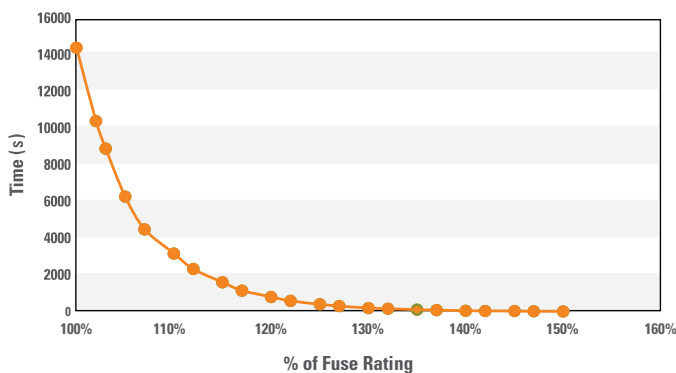
High Current Interrupt Time (100-150%)
