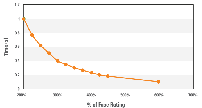
High Current Interrupt Time (200-600%)
