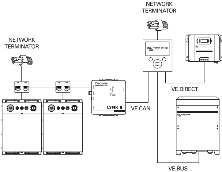
Figure 1. Example LYNK II with Victron Energy devices
