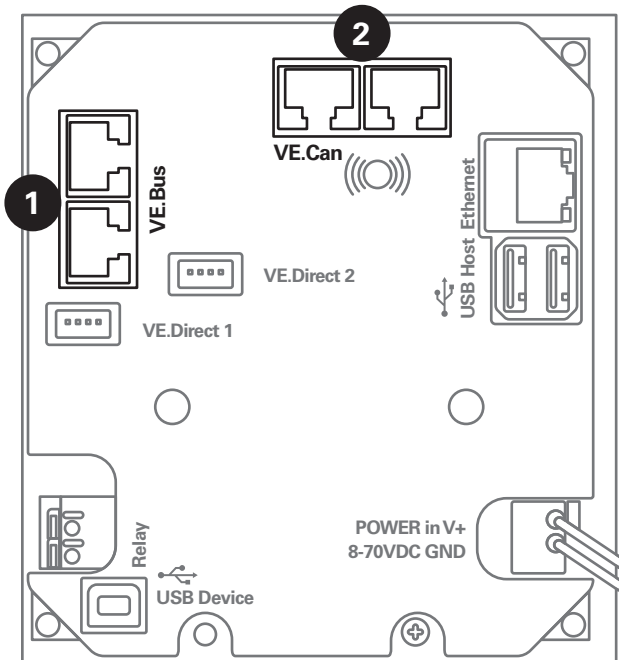
Figure 6. Victron GX device
