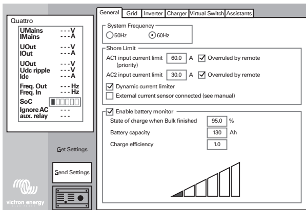
Figure 7. VE Configure 3 Software
